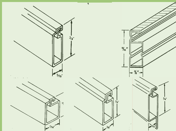
SCREEN FRAME: Roll Formed Aluminum
